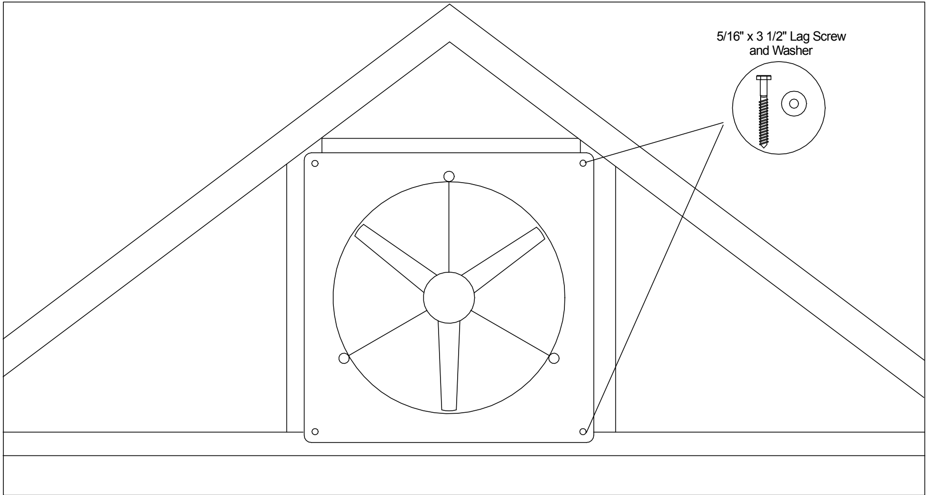
Installation for 12", 16" & 20" Snap-Fan
